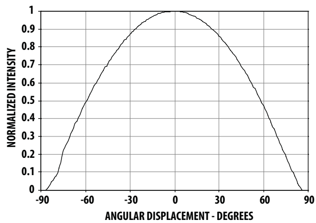
Figure 6. Radiation pattern.
