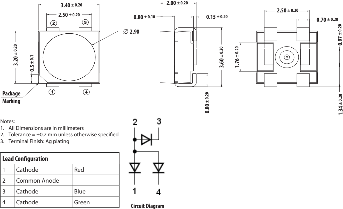
Figure 1. Package drawing
