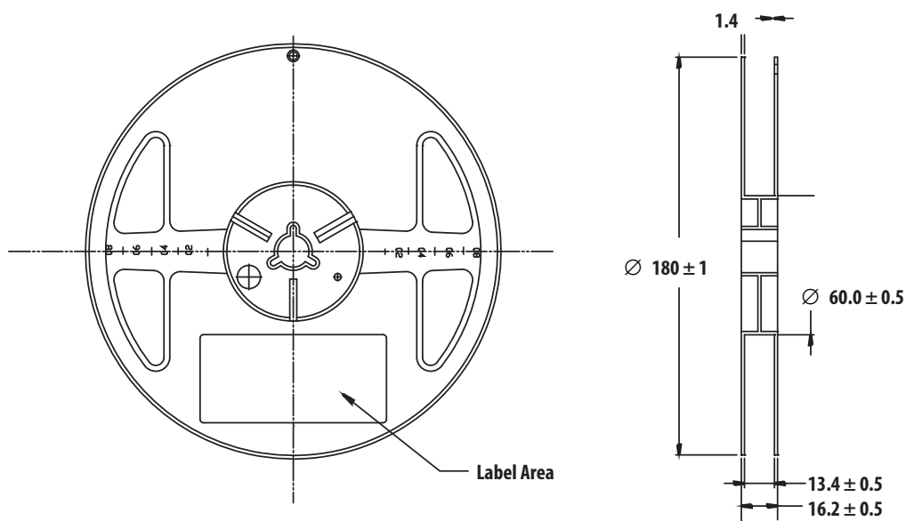
Figure 14. Reel Dimension
