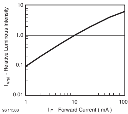
Figure 6. Relative Luminous Intensity vs. Forward Current
