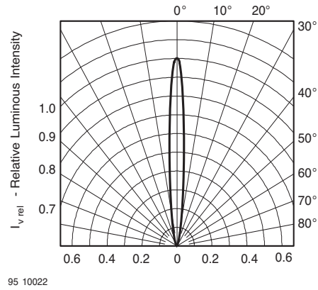
Figure 3. Rel. Luminous Intensity vs. Angular Displacement
