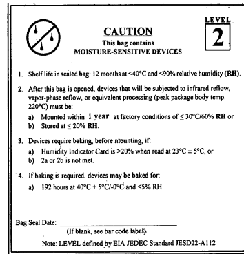
Example of JESD22-A112 Level 2 label
