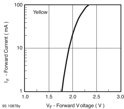
Figure 14. Forward Current vs. Forward Voltage
