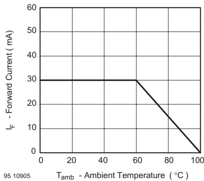
Figure 2. Forward Current vs. Ambient Temperature for InGaN
