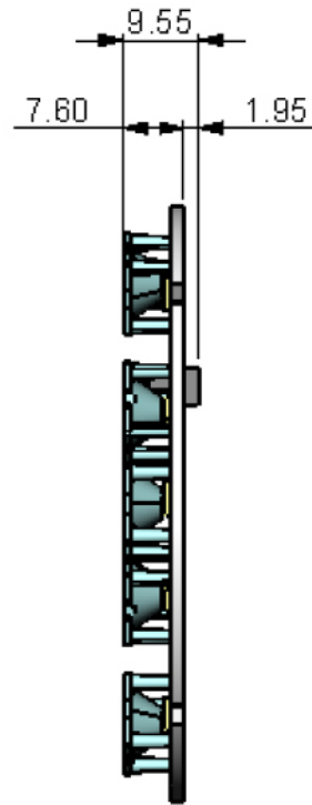
PCB WITH 10mm OPTIC
