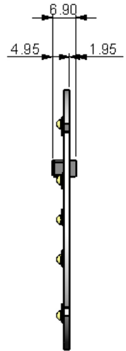
PCB WITHOUT OPTIC
