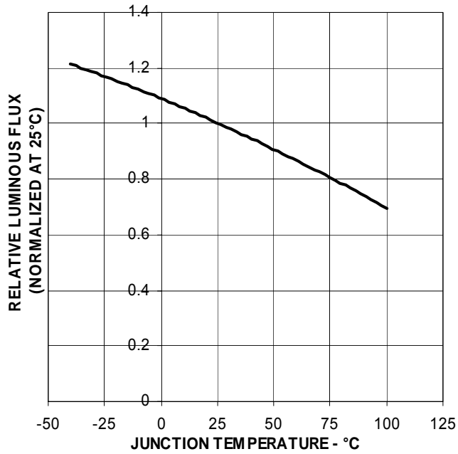
Figure 5. Relative Intensity Vs. Temperature
