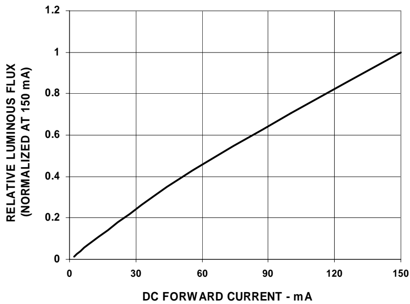
Figure 4. Relative Flux vs. Forward Current
