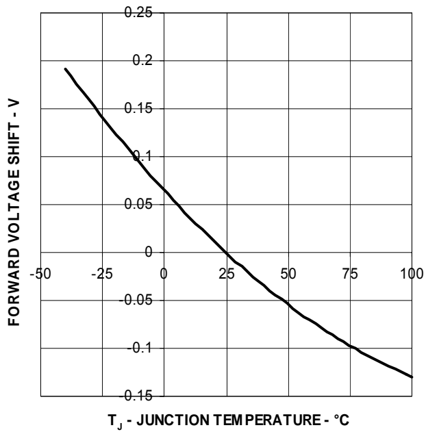
Figure 7. Forward Voltage Shift Vs. Temperature.
