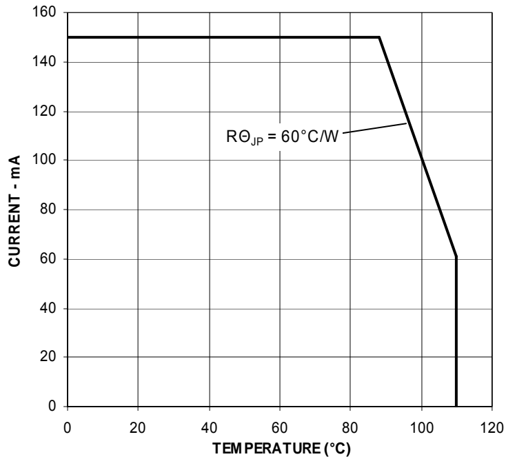
Figure 6b. Maximum Forward Current Vs. Solder Point Temperature. Derated Based on T_{JMAX} = 125^{\circ}C , R\theta_{J-P} = 60^{\circ}C/W .
