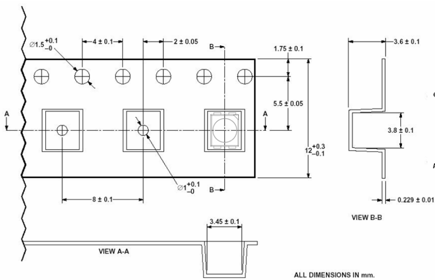
Figure 13. Tape Dimensions.
