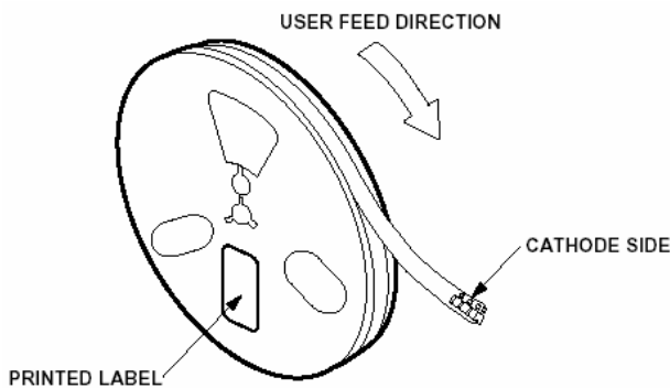
Figure 14. Reeling Orientation.
