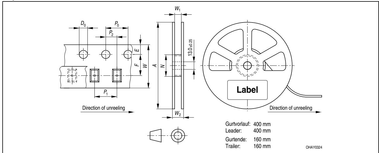
Tape dimensions in mm (inch)
