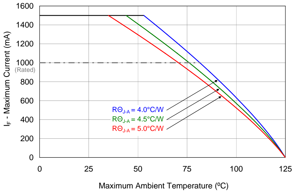
Figure 8: Maximum forward current vs. ambient temperature based on T J(MAX) = 125°C.
