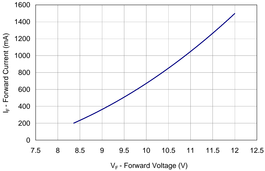
Figure 7: Typical forward current vs. forward voltage @ T c = 25°C.
