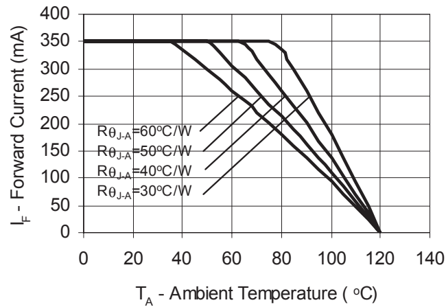
Figure 5b. Maximum Forward Current vs. Ambient Temperature. Derating based on T_{JMAX} = 120^\circ\text{C} for Warm White.
