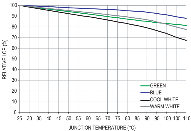
Figure 9. Relative LOP vs. junction temperature
