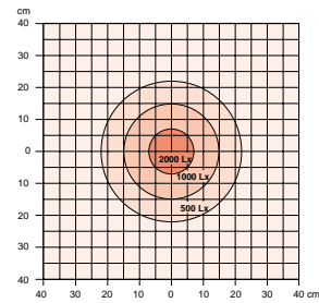
Luminous intensity/Lux rating – Sunnex HM 35W
