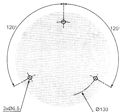
Panel cut-out
