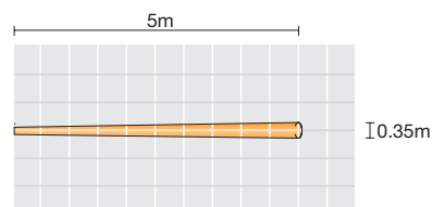
WolfLite H-251A 2.8w spot beam (approx 4°) Peak luminous intensity at 5m 700lux
