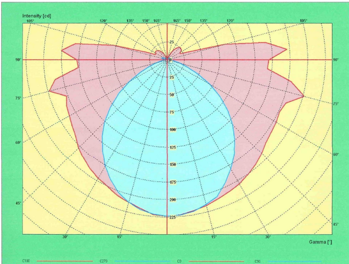
YD630MM Non-maintained emergency bulkhead light 070809PA
