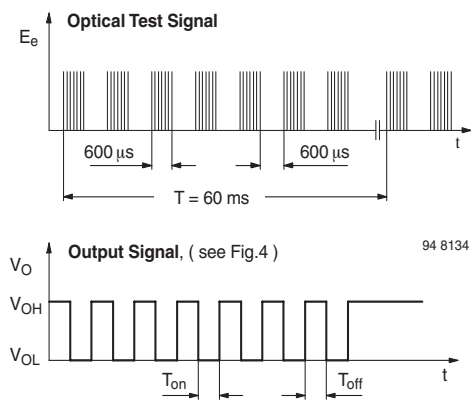
Figure 3. Output Function
