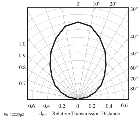
Figure 12. Directivity
