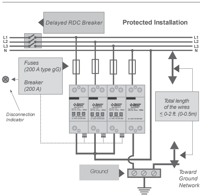
Parallel Connection
