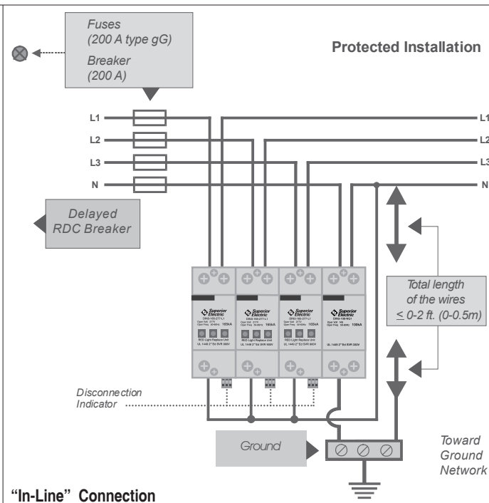
"In-Line" Connection
