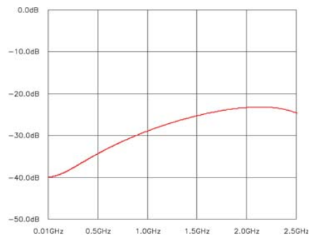
Figure 3 Typical return loss for N-type CA devices
