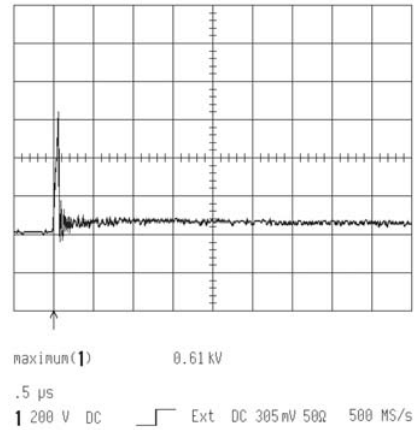
Figure 1 Typical limiting voltage for the CA350
