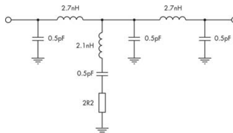
Figure 4 Equivalent circuit diagram
