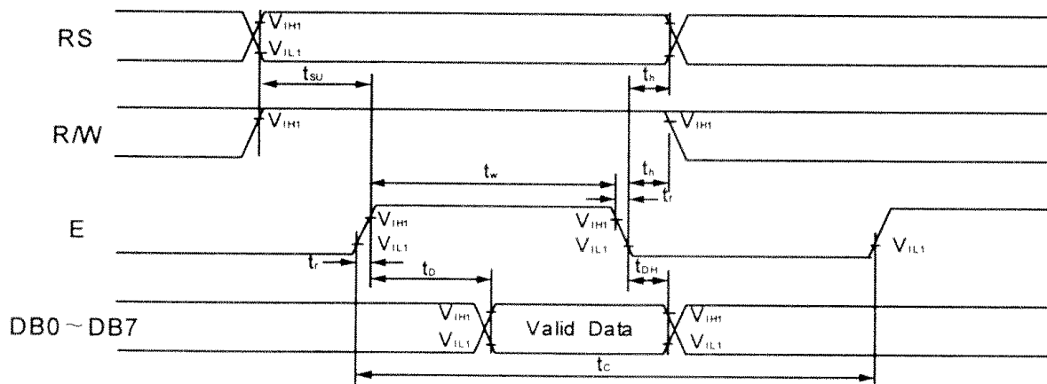
Figure 3: Write Mode Timing Diagram
