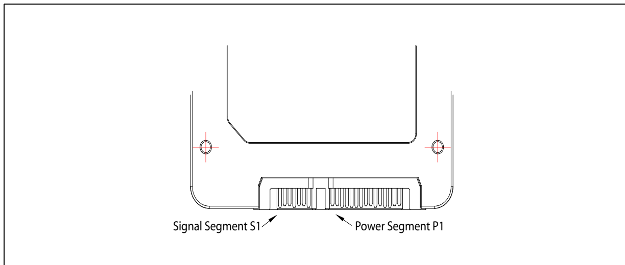
Figure 7. Layout of Signal and Power Segment Pins
