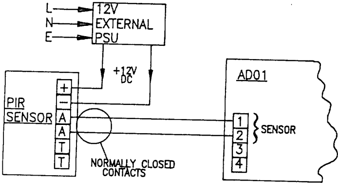
Fig1 PIR CONNECTION TO AD01
