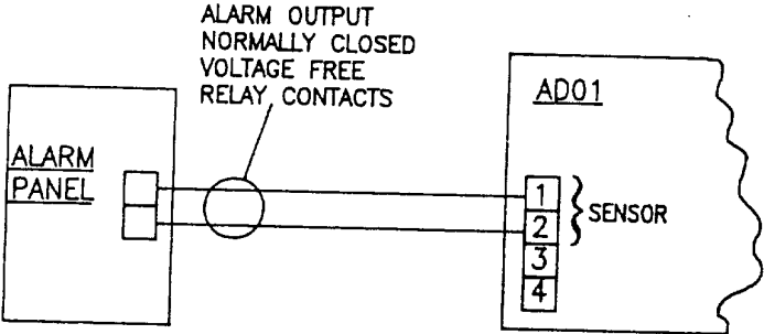
Fig2 ALARM PANEL CONNECTION TO AD01
