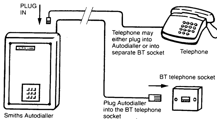
FIGURE 1. Autodialler Installation
