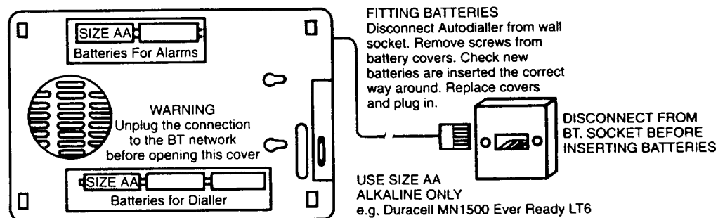
FIGURE 2. Fitting the Batteries
