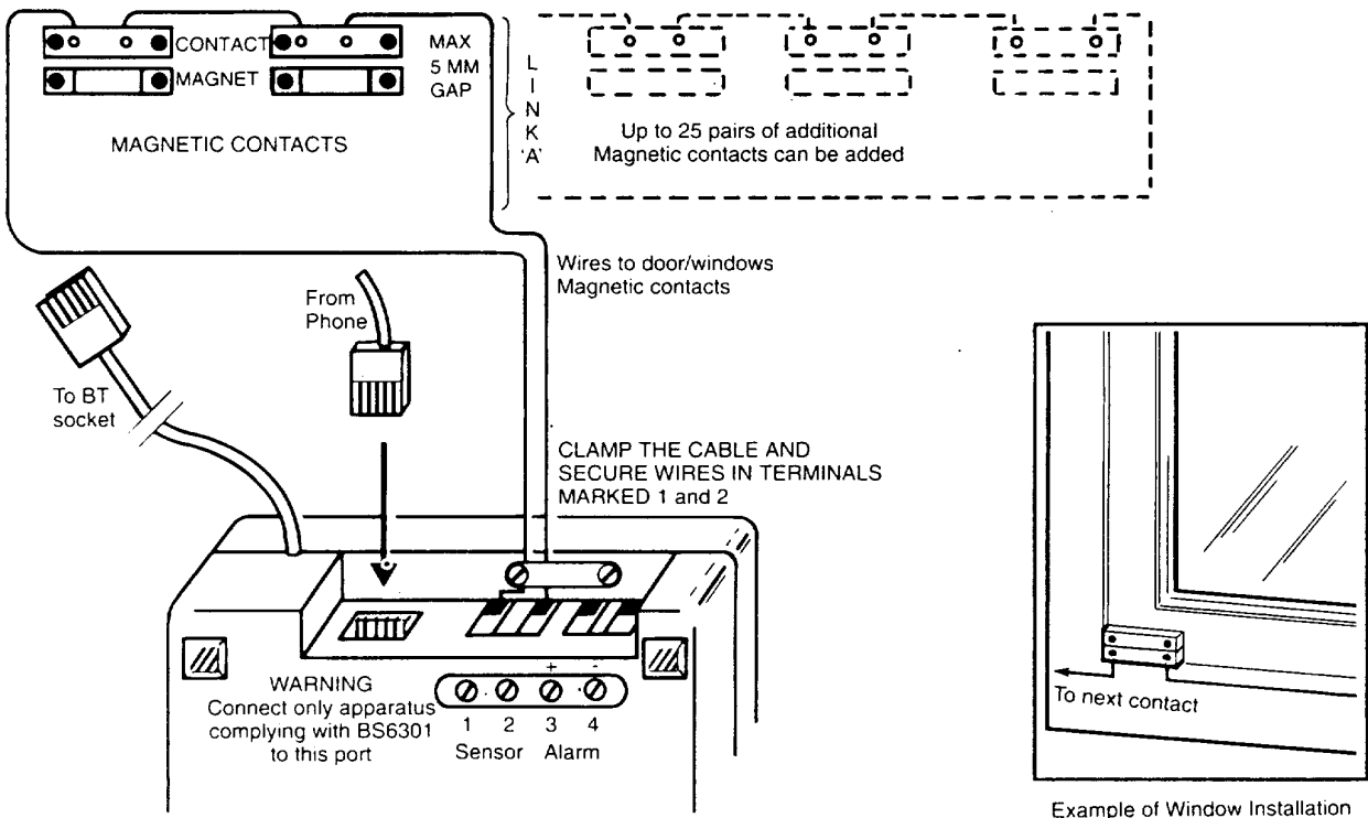
FIGURE 3. Installing the Magnetic Door/Window contacts
