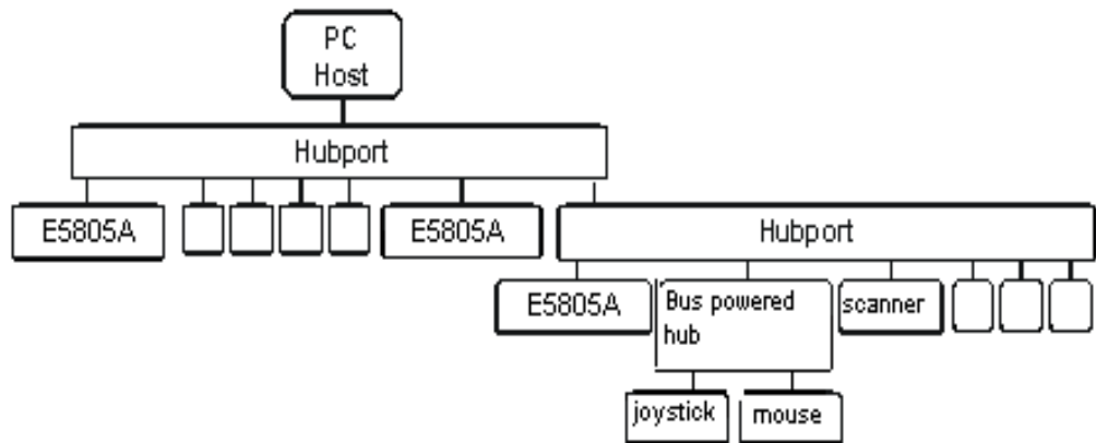
Figure 1 Hub Architecture
