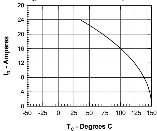
Fig. 5. Drain vs. Case Temperature
