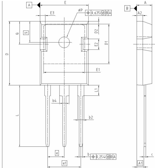
PG-TO247-3-21
