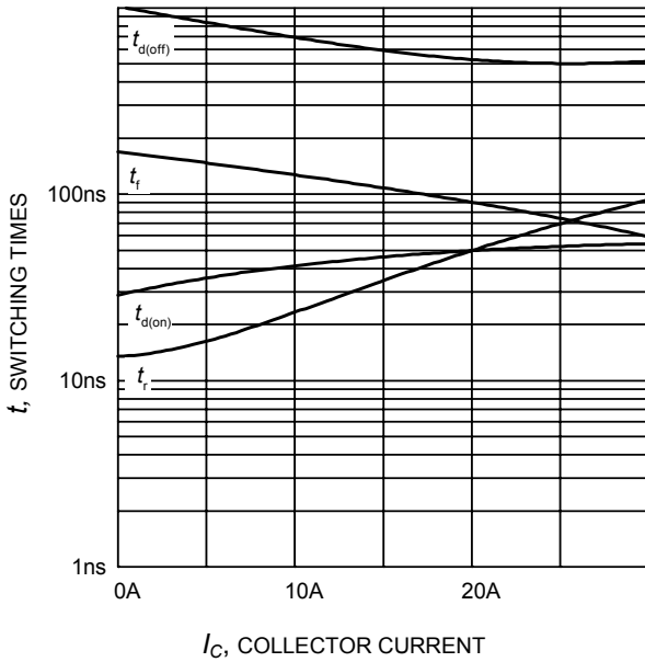
Figure 9. Typical switching times as a function of collector current (inductive load, T_J=150^{\circ}\text{C} , V_{CE}=600\text{V} , V_{GE}=0/15\text{V} , R_G=56\Omega , Dynamic test circuit in Figure E)
