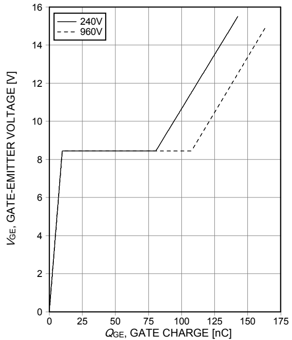
Figure 18. Typical gate charge ( I_c=15A )
