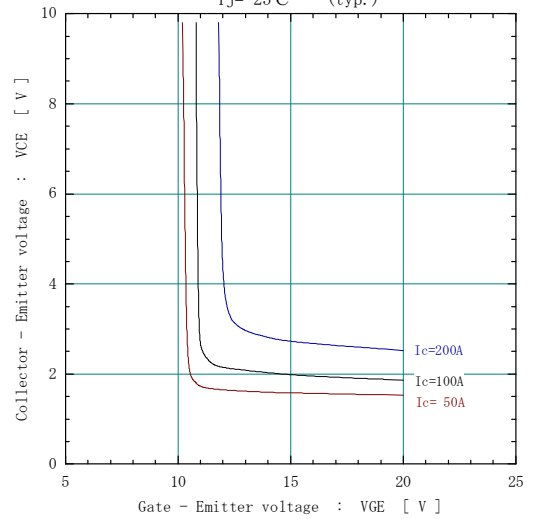
[ Inverter ] Collector-Emmitter voltage vs. Gate-Emmitter voltage Tj= 25°C (typ.)
