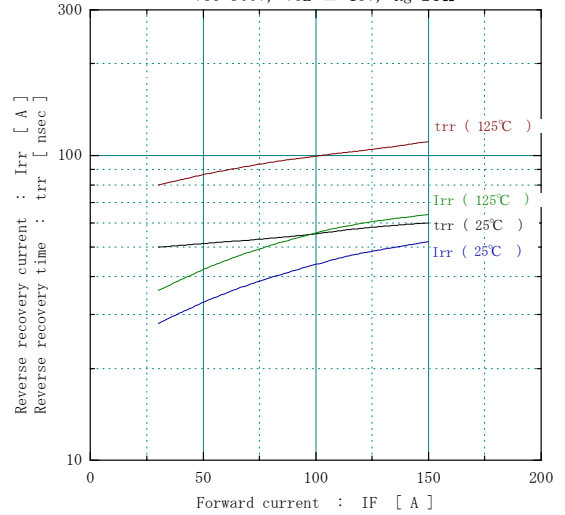
[ Inverter ] Reverse recovery characteristics (typ.) Vcc=300V, VGE=±15V, Rg=24Ω
