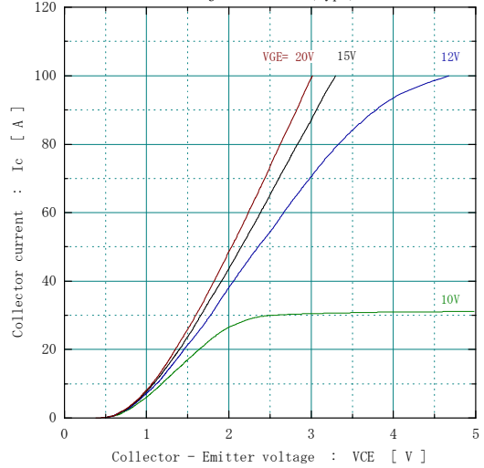
[ Brake ] Collector current vs. Collector-Emitter voltage Tj= 125°C (typ.)
