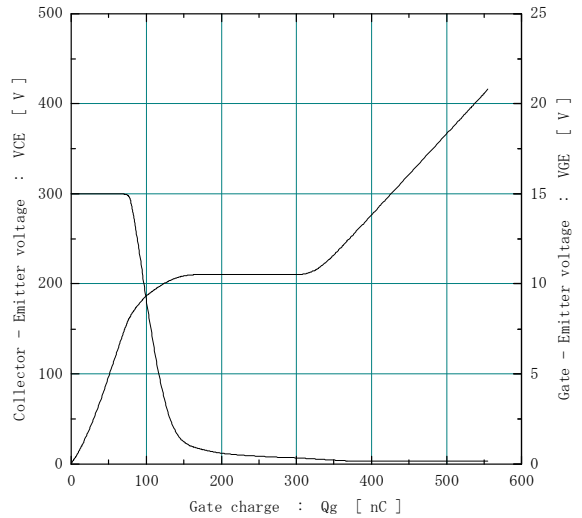
[ Inverter ] Dynamic Gate charge (typ.) Vcc=300V, Ic=100A, Tj= 25°C
