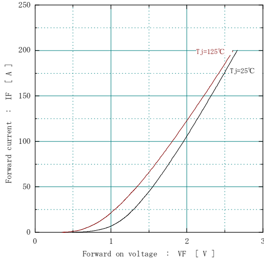
[ Inverter ] Forward current vs. Forward voltage (typ.)
