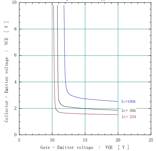
[ Brake ] Collector-Emitter voltage vs. Gate-Emitter voltage Tj= 25°C (typ.)
