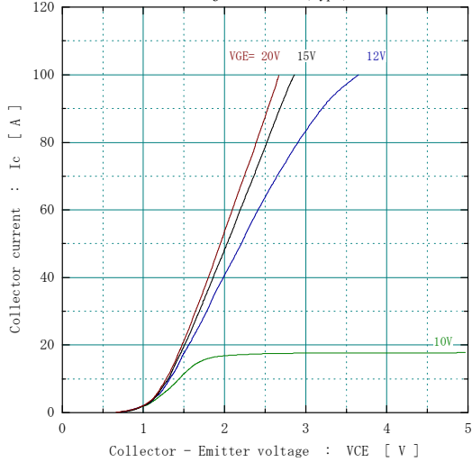
[ Brake ] Collector current vs. Collector-Emitter voltage Tj= 25°C (typ.)
