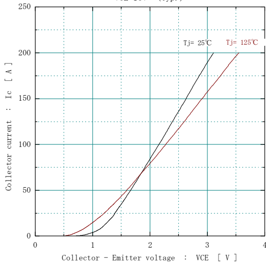
[ Inverter ] Collector current vs. Collector-Emmitter voltage VGE=15V (typ.)
