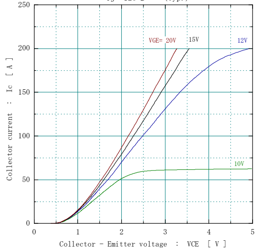
[ Inverter ] Collector current vs. Collector-Emmitter voltage Tj= 125°C (typ.)
