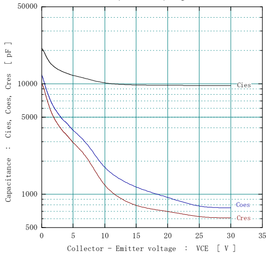
[ Inverter ] Capacitance vs. Collector-Emmitter voltage (typ.) VGE=0V, f= 1MHz, Tj= 25°C
