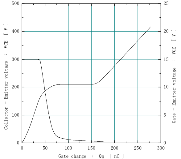
[ Brake ] Dynamic Gate charge (typ.) Vcc=300V, Ic=50A, Tj= 25°C
