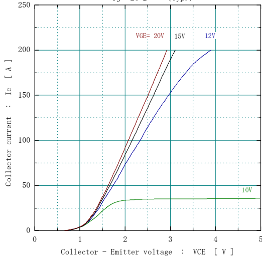
[ Inverter ] Collector current vs. Collector-Emmitter voltage Tj= 25°C (typ.)
