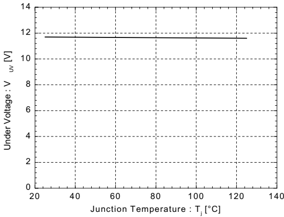
Under Voltage vs. Junction Temperature
