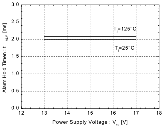
Alarm Hold Time vs. Power Supply Voltage
