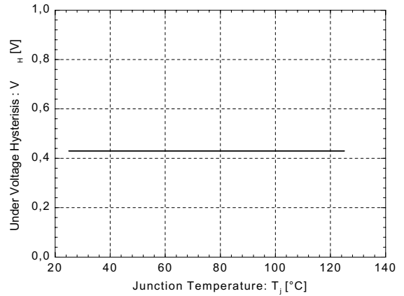
Under Voltage Hysteresis vs. Junction Temperature
