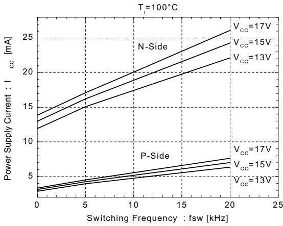
Power Supply Current vs. Switching Frequency
