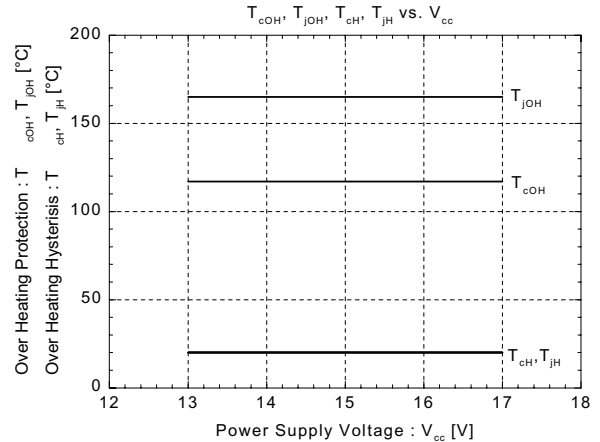
Over Heating Characteristics
