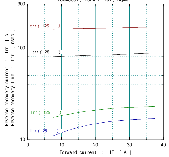
Reverse recovery characteristics (typ.) Vcc=600V, VGE=± 15V, Rg=51
