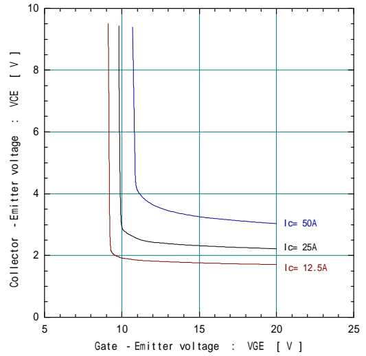
Collector-Emmitter voltage vs. Gate-Emmitter voltage Tj= 25 (typ.)
