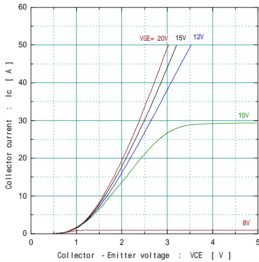
Collector current vs. Collector-Emmitter voltage Tj= 25 (typ.)
