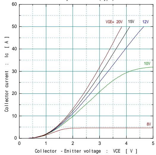
Collector current vs. Collector-Emmitter voltage Tj= 125 (typ.)
