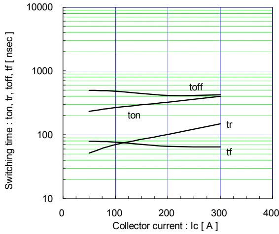
Switching time vs. Collector current (typ.) V_{CC}=600V, V_{GE}=\pm 15V, R_G=3.0\Omega, T_J=25^\circ C
