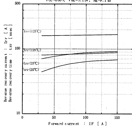
Reverse recovery characteristics (typ.) Vcc=600V, VGE=±15V, Rg=9.1Ω
