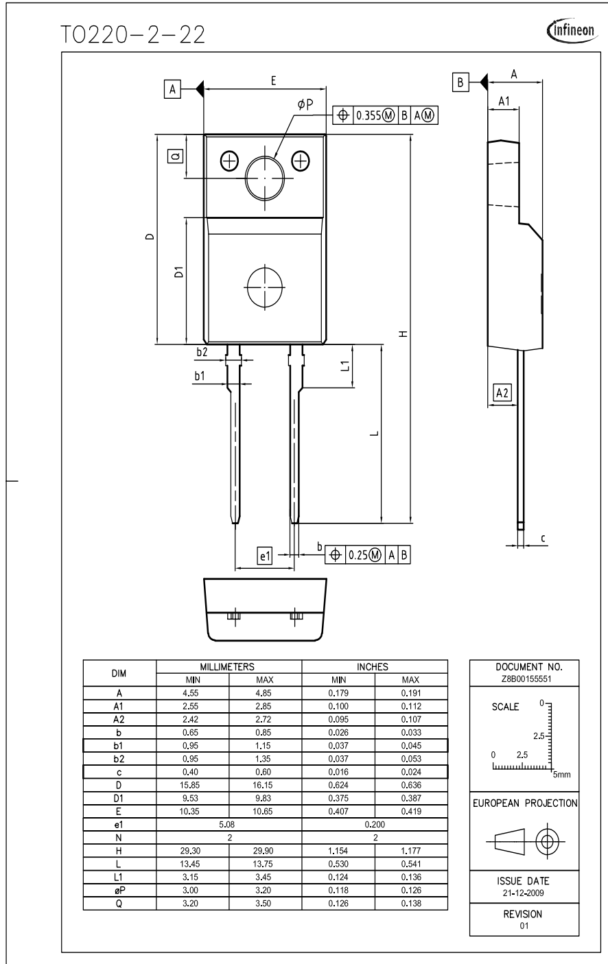
Figure 1 Outlines TO-220 FullPAK, dimensions in mm/inches
