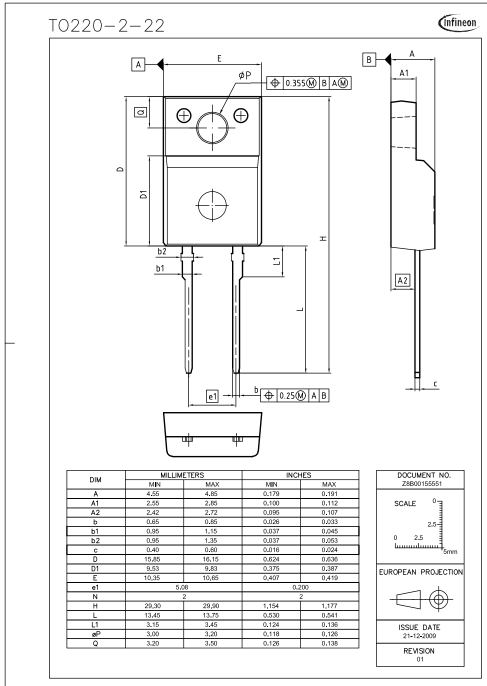
Figure 1 Outlines TO-220 FullPAK, dimensions in mm/inches
