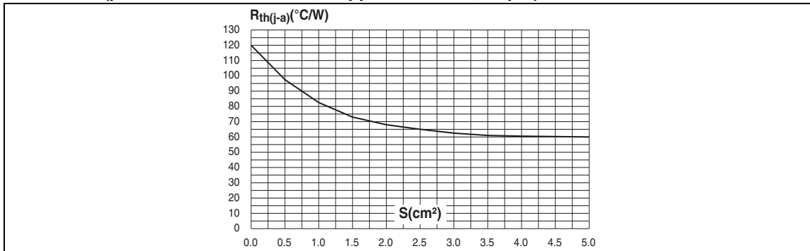
Figure 11. SOT-223 thermal resistance junction to ambient versus copper surface under case (printed circuit board FR4, copper thickness; 35 μm)
