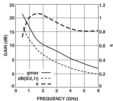
Figure 11. Gain vs. Frequency at 2.7V, 5mA.
