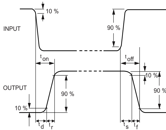
Figure 1. Switching Waveform
