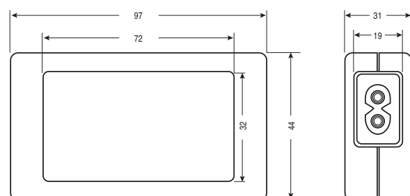
MECHANICAL DIMENSIONS (mm)
