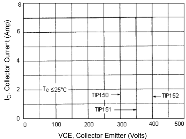
Reverse Biase Safe Operating Area
