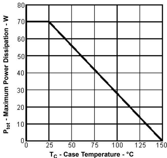
Maximum Power Dissipation vs Case Temperature
