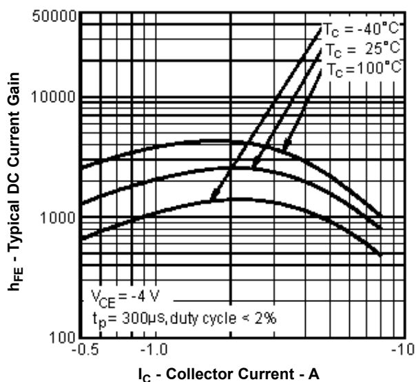
Typical DC Current Gain vs Collector Current
