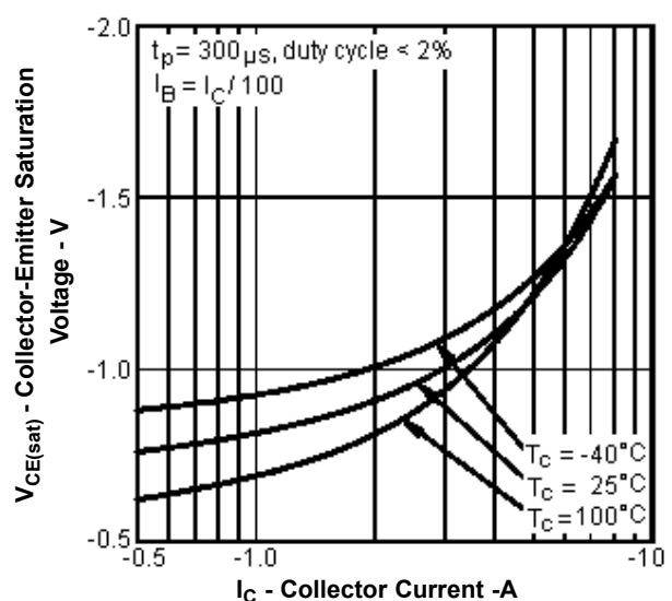
Collector-Emitter Saturation Voltage vs Collector Current
