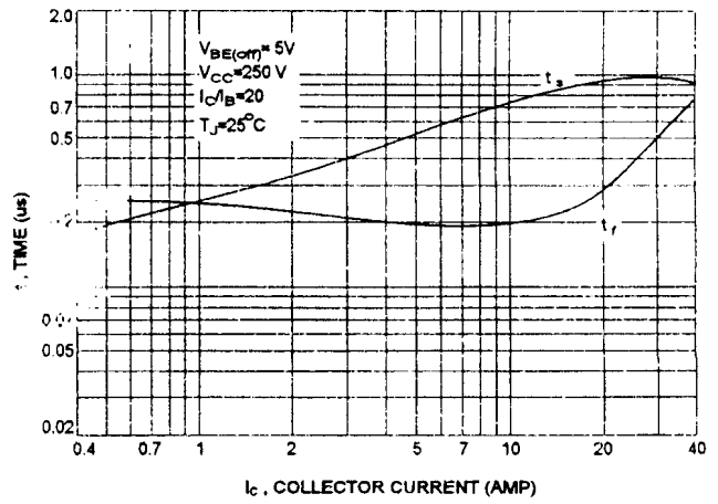
TURN-OFF TIME
