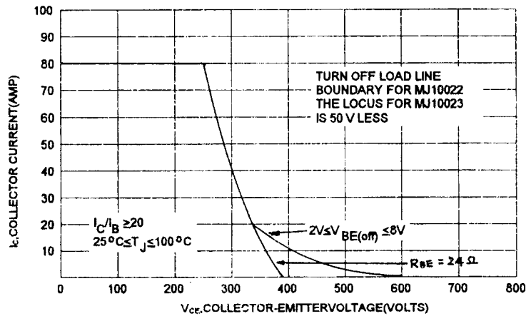
REVERSE BIAS SWITCHING SAFE OPERATING AREA
