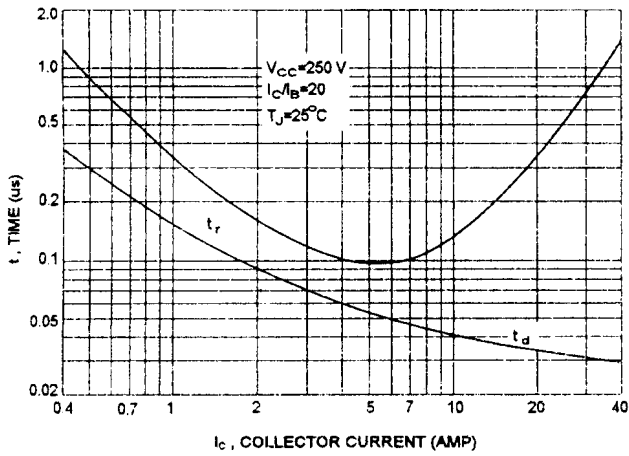
TURN-ON TIME
