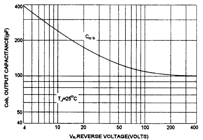
OUTPUT CAPACITANCES
