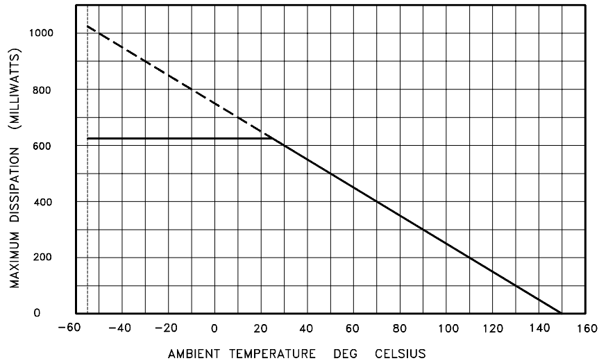
DERATING CURVE
