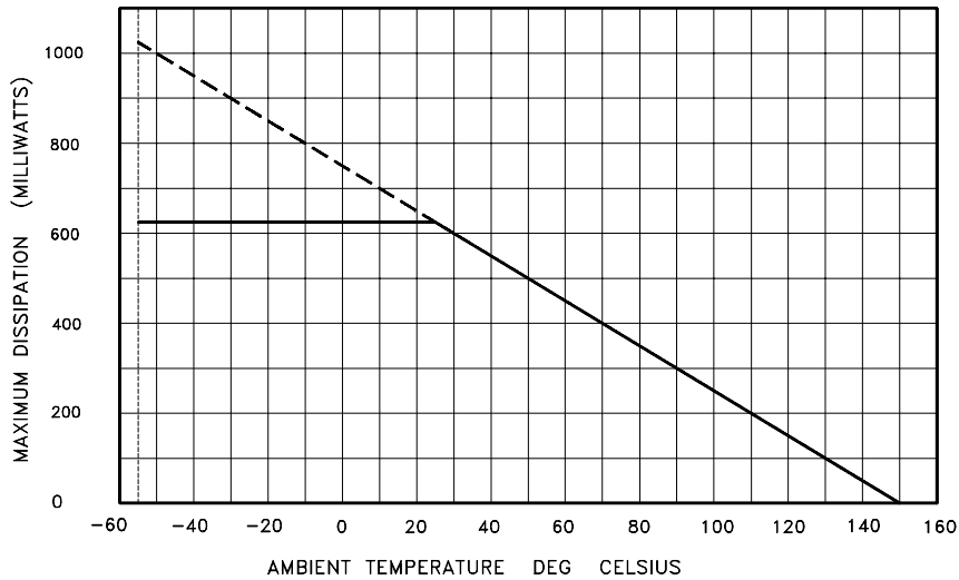
DERATING CURVE
