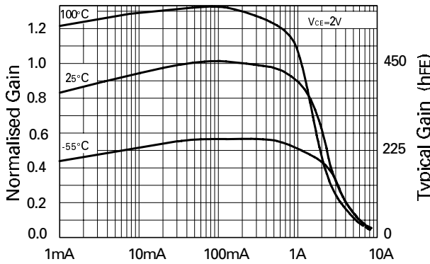
Collector Current
