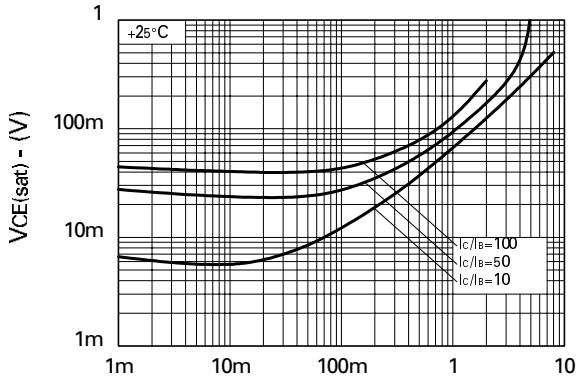
IC - Collector Current (A)
