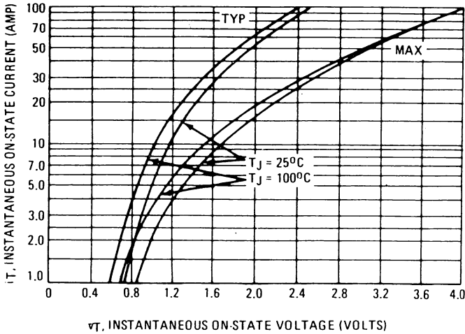
FIGURE 8 – FORWARD VOLTAGE
