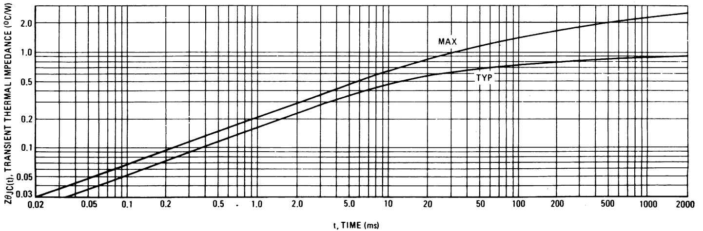
FIGURE 7 – THERMAL RESPONSE
