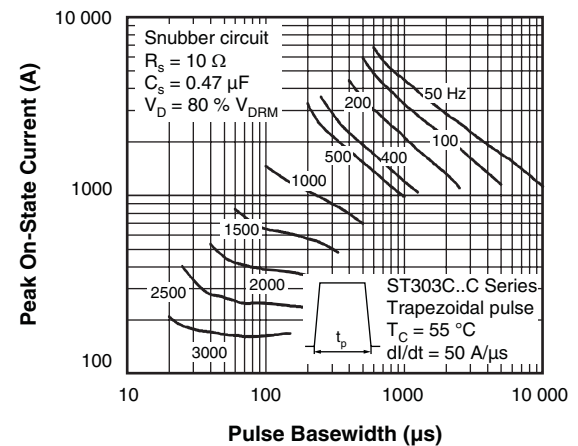
Fig. 14 - Frequency Characteristics
