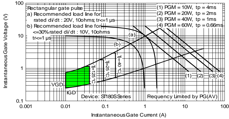
Fig. 9 - Gate Characteristics
