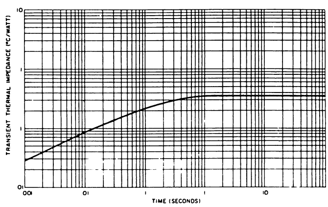
8. TRANSIENT THERMAL IMPEDANCE – JUNCTION-TO-CASE
