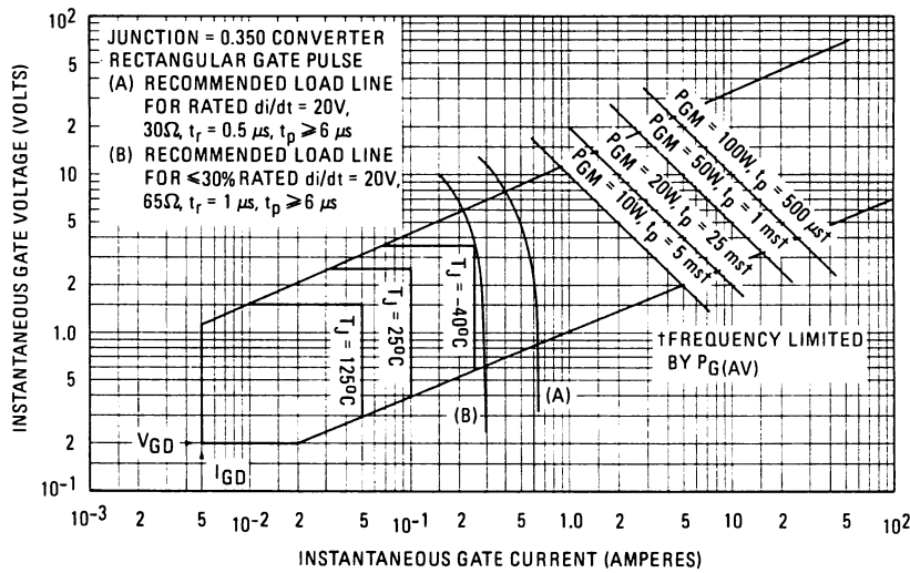
Fig. 9 – Gate Characteristics
